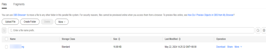
Figure 12-1 File list
