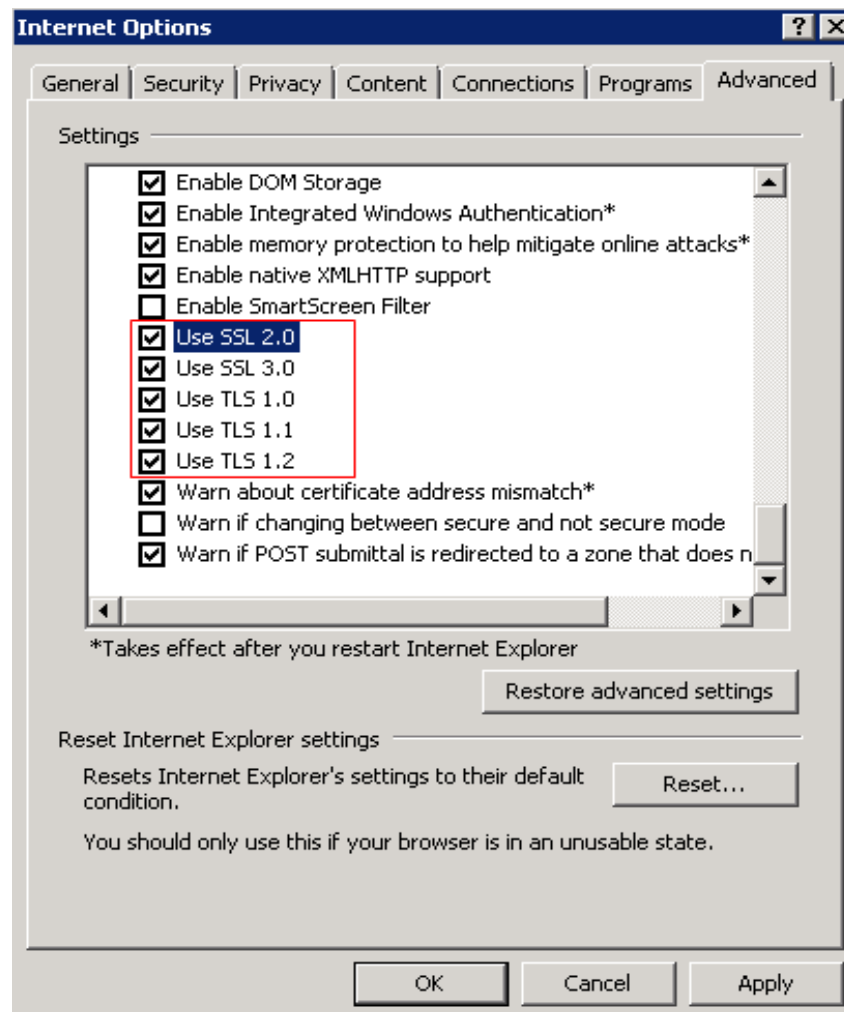
Figure 14-1 Internet Options
